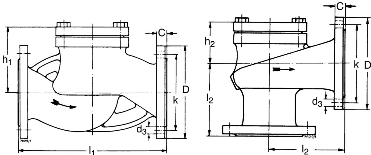
Straight-way valve
