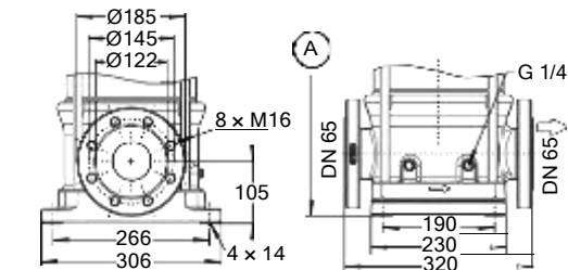
Fig. 52: Movitec VCF; DN 65
