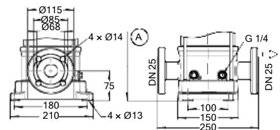
Fig. 8: Movitec VCF
