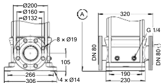
Fig. 47: Movitec VF, VSF - interchangeable range
