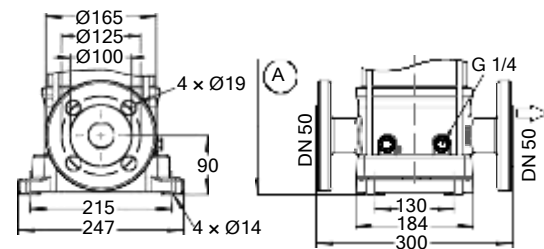
Fig. 36: Movitec VCF
