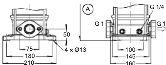
Fig. 4: Movitec V, VS
