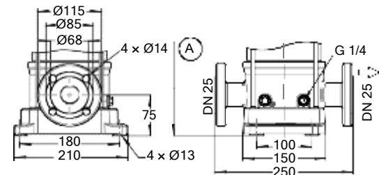
Fig. 14: Movitec VCF
