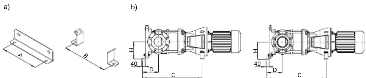
Fig. 70: a) Pump bracket b) Pump set
