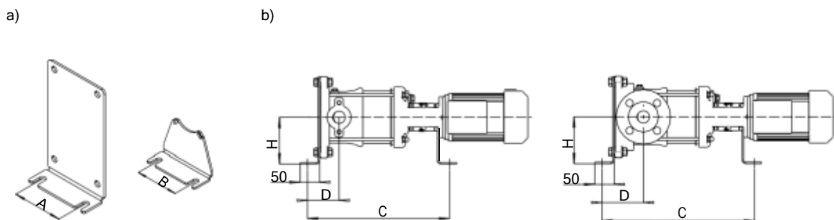
Fig. 69: a) Pump bracket b) Pump set
