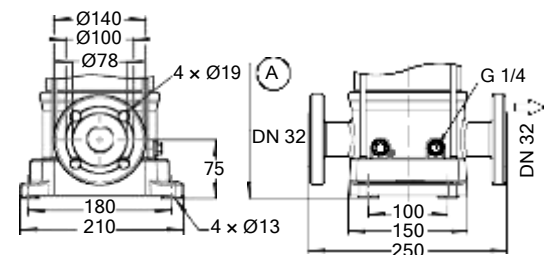
Fig. 20: Movitec VCF
