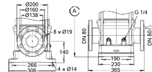
Fig. 53: Movitec VCF; DN 80
