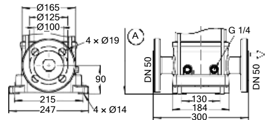
Fig. 41: Movitec VCF
