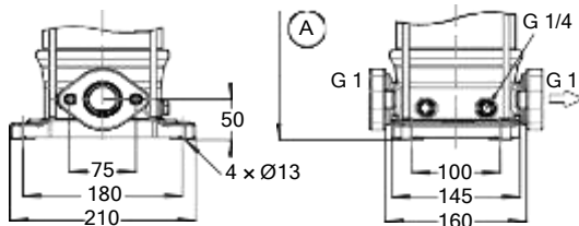
Fig. 10: Movitec V, VS
