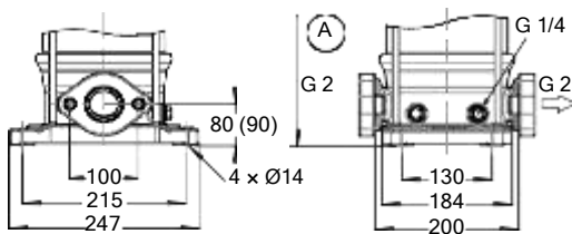
Fig. 32: Movitec V, VS
