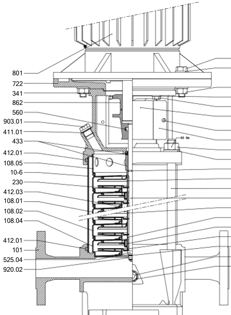
Fig. 77: General assembly drawing of Movitec LHS 6
